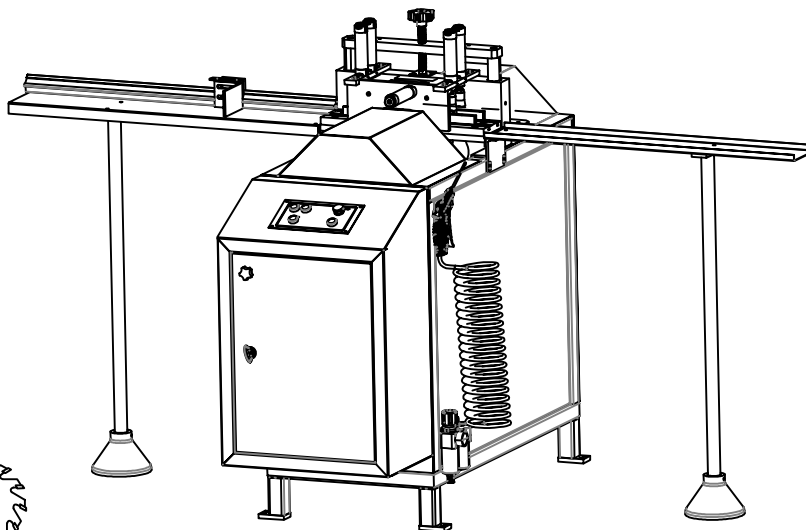
250 mm BLADE X 2 ID 30 mm
